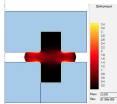
Fig. 2. The scheme of combined extrusion
